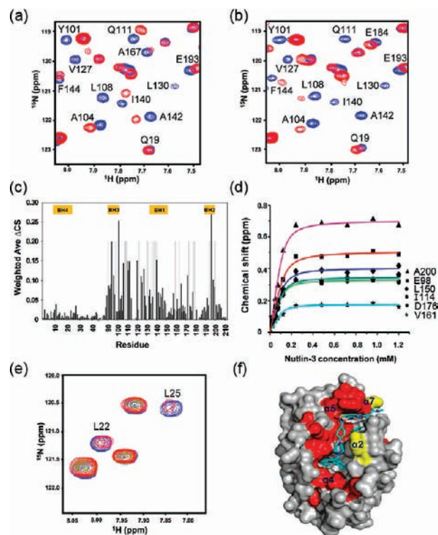
Figure 4. Binding of Nutlin-3 and PMI to anti-apoptotic Bcl-X L . (a, b) Overlaid 2D 1 H– 15 N HSQC spectra for 15 N-labeled Bcl-X L in the absence (blue) and presence (red) of (a) Nutlin-3 and (b) PMI. (c) Chemical shift perturbations of Bcl-X L upon binding to Nutlin-3. Resonances that disappeared upon binding are shown as gray bars. (d) Plots of chemical shift changes in Bcl-X L resonances induced by Nutlin-3. (e) Displacement of 15 N-labeled p53TAD from Bcl-X L by the addition of Nutlin-3 (red). The blue cross-peaks represent NMR resonances for free 15 N-labeled p53TAD, and the green cross-peaks represent those for 15 N-labeled p53TAD bound to Bcl-X L . (f) Chemical shift perturbations of Bcl-X L induced by Nutlin-3 mapped onto the structure of Bcl-X L complexed with ABT-737. The Bcl-X L residues showing chemical shift changes of ΔCS > 0.2 are colored yellow, and residues for which the cross-peaks disappeared upon binding of Nutlin-3 are colored red.
