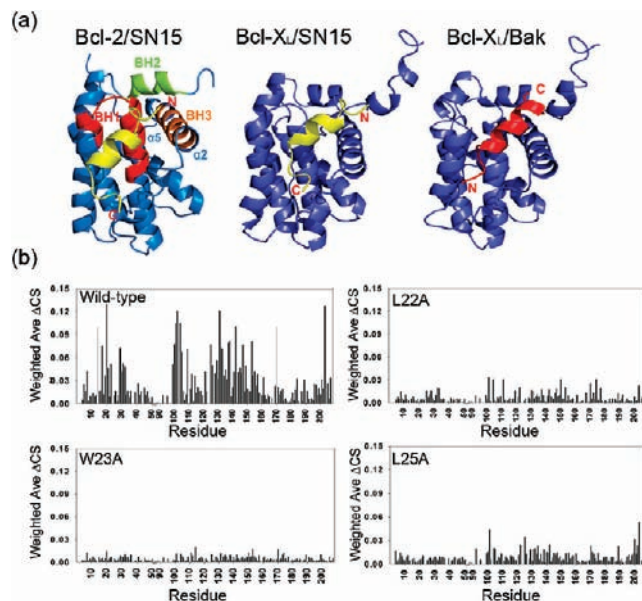
Figure 2. Structural model for the Bcl-2/SN15 peptide complex. (a) Structural models of the Bcl-2/SN15 and Bcl-X L /SN15 complexes compared with the crystal structure of the Bcl-X L /Bak complex. The SN15 and Bak peptides are shown in yellow and red, respectively. (b) Chemical shift perturbations of Bcl-2 residues upon binding to the alanine mutants of SN15. Resonances that disappeared upon binding are shown as gray bars.
