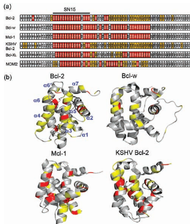
Figure 1. Binding site mapping of the interaction between the p53TAD and anti-apoptotic Bcl-2 family proteins. (a) Sequence-based chemical shift perturbation maps of the p53TAD upon binding to Bcl-2 family proteins and MDM2. The red-colored region indicates cross-peaks of the p53TAD that disappeared or were weakened upon binding, whereas the orange-colored region shows cross-peaks that moved. The cross-peaks that remained unaffected by binding and prolines are shown in white and gray, respectively. (b) SN15 peptide-binding site mapped on Bcl-2 family proteins. The residues showing chemical shift changes with \Delta\text{CS} > 0.08 and 0.03 < \Delta\text{CS} < 0.08 are colored red and yellow, respectively.
