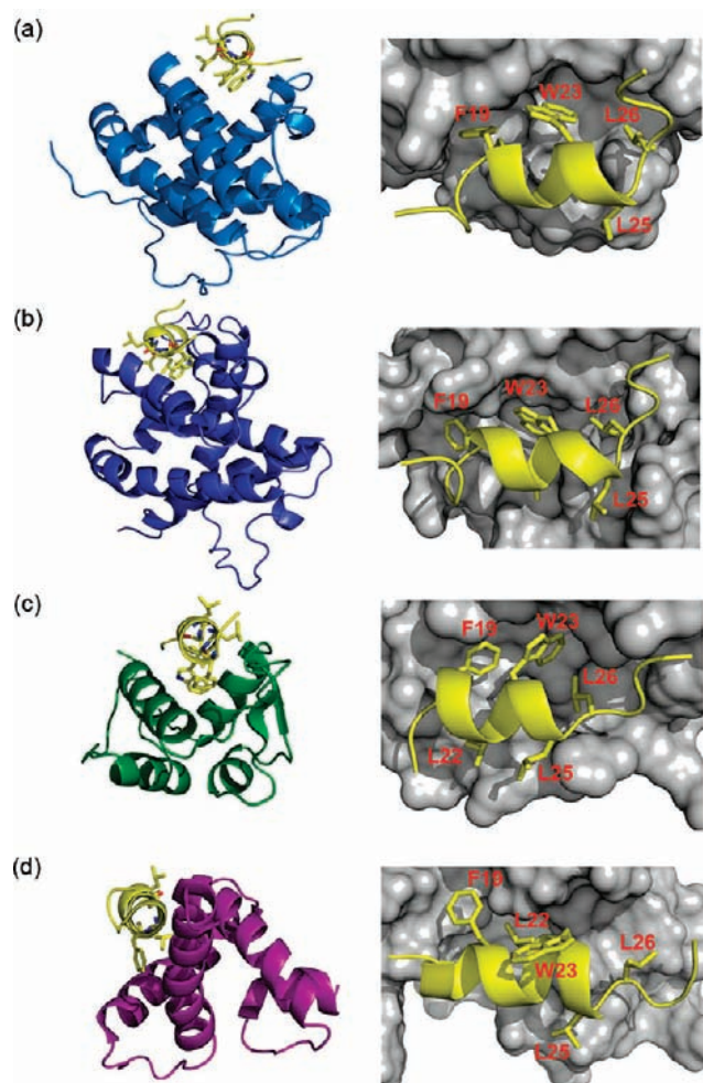
Figure 3. Mimicry in the recognition of anti-apoptotic Bcl-2 family proteins and MDM2 by the p53TAD. Structural models of the (a) Bcl-2/SN15 and (b) Bcl-X L /SN15 complexes were compared with the previously reported structures of the (c) MDM2/SN15 and (d) p300 Taz2/SN15 complexes. The SN15 peptides are drawn as yellow ribbon models, and the residues involved in binding are labeled.
